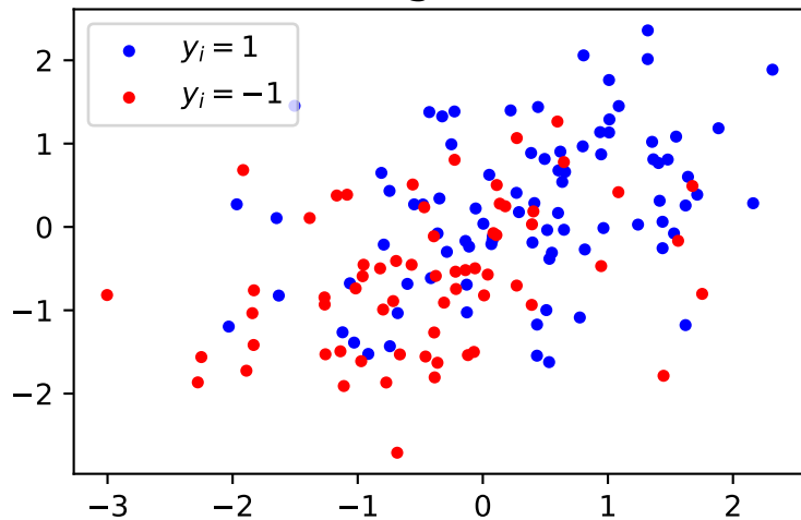
Logistic
