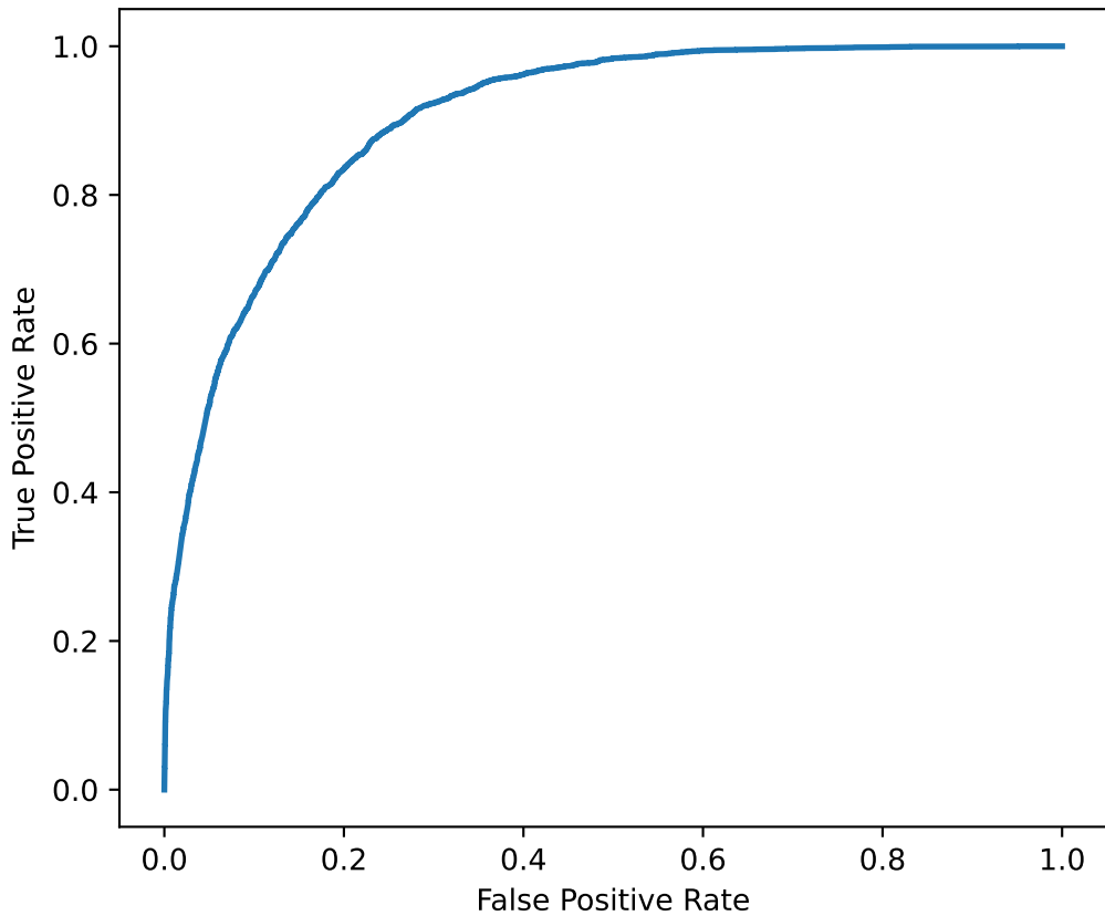
ROC curve on adult dataset (area = 0.90)
