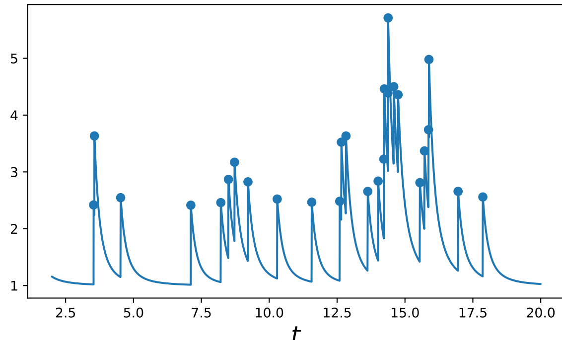
ticks #0, t \in [2, 20]
