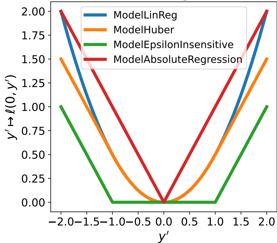
Losses for regression
