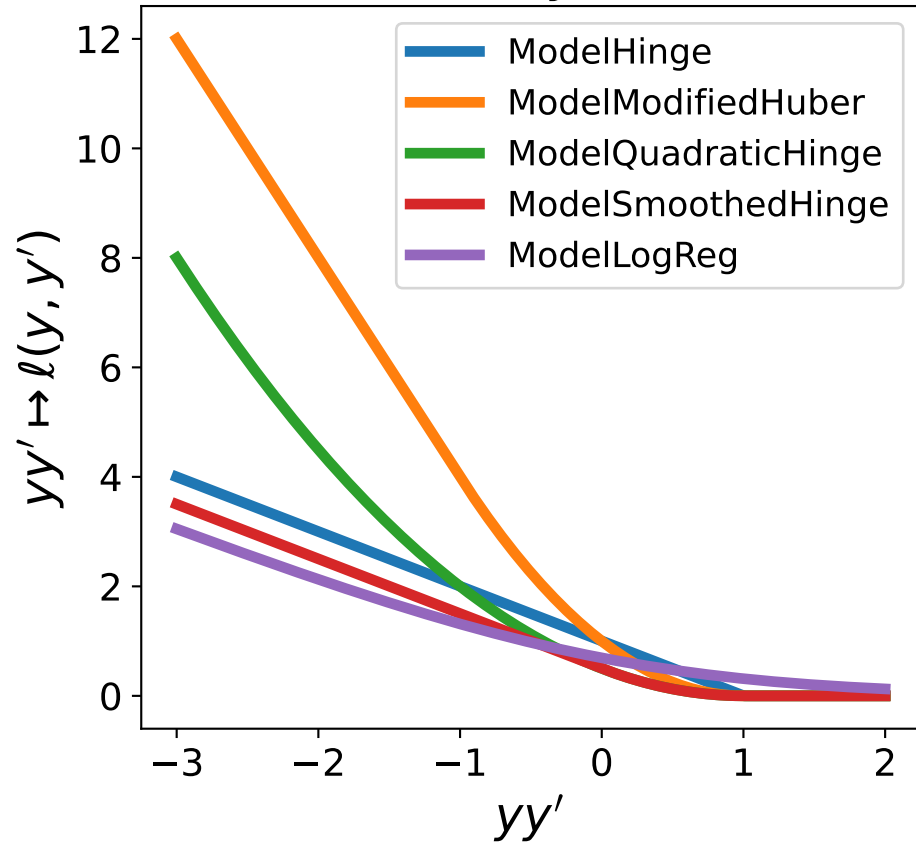
Losses for binary classification
