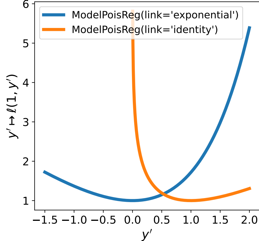
Losses for count data
