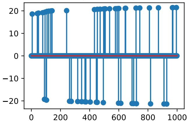
Sample intercepts
