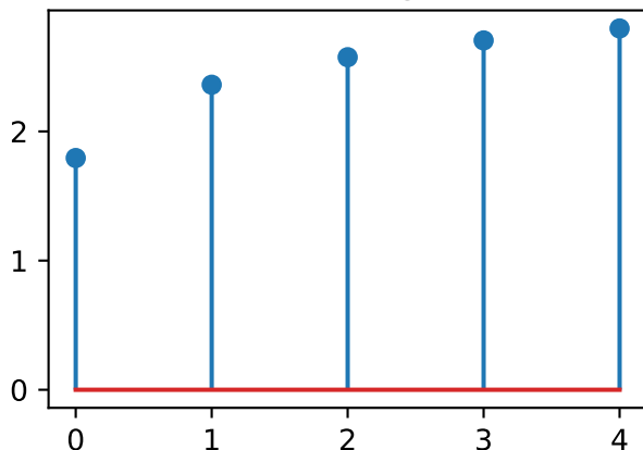
Model weights
