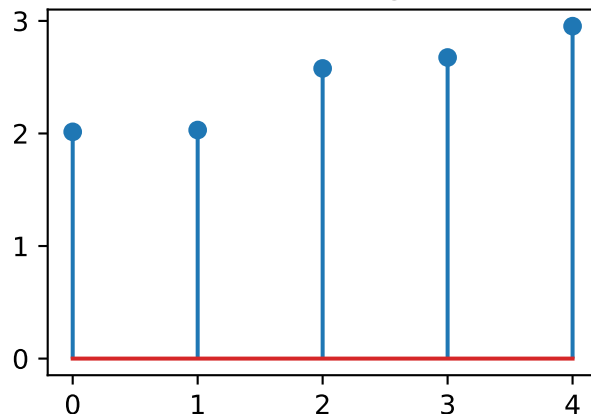
Learned weights
