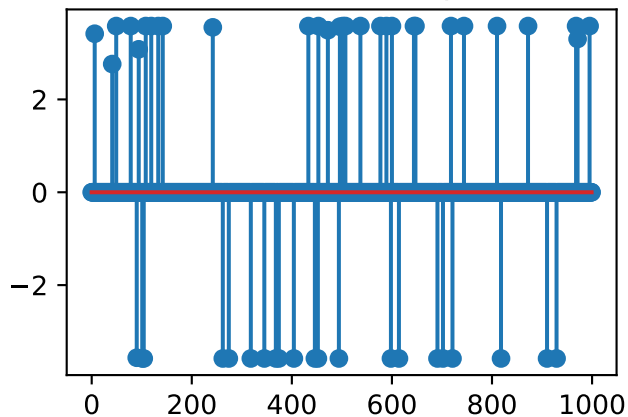
Learned intercepts
