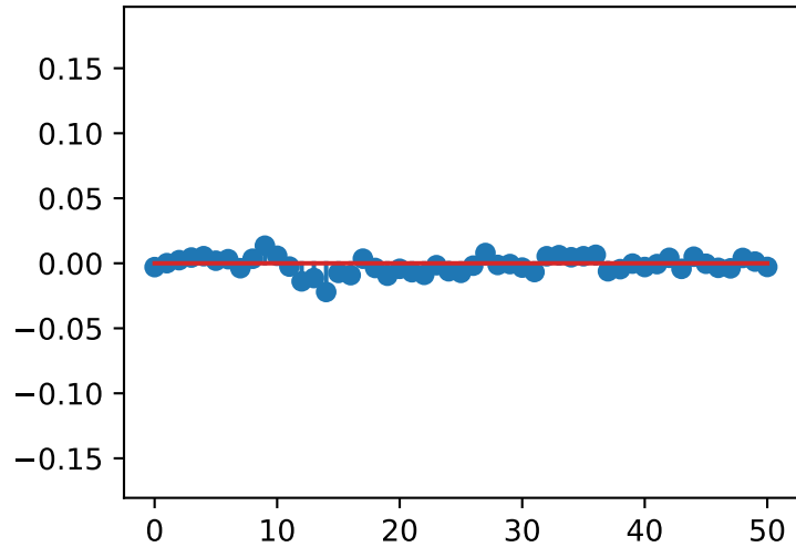
\nabla f(\text{coeffs0})
