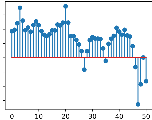
\nabla f(\text{coeffs1})
